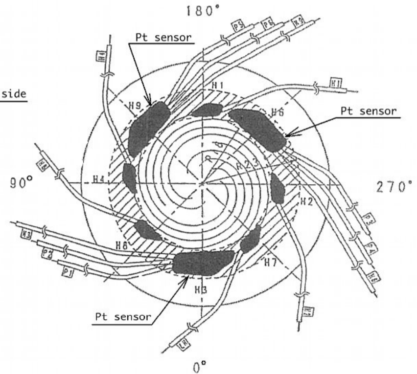
Heater side
