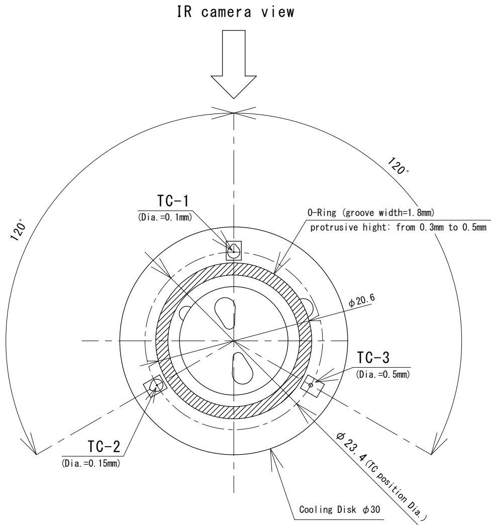
TC layout on Cooling Disk
