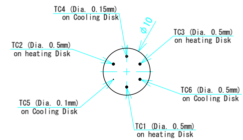
TC layout, perspective view from the cooling disk side
