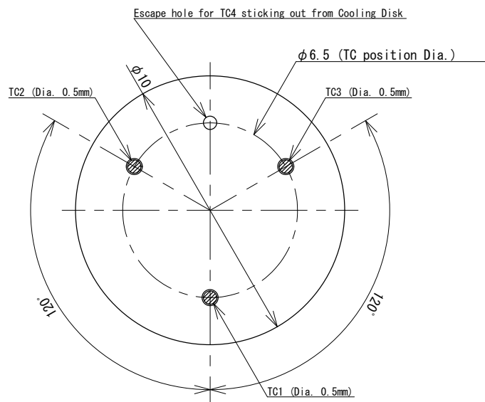
TC layout on Heating Disk View from the cooling disk side
