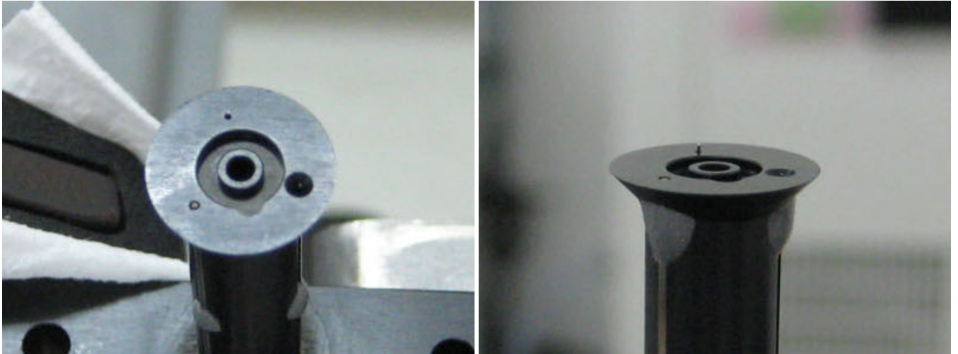
Cooling Disk Photos without O-Ring The center hole is where liquid comes out.
