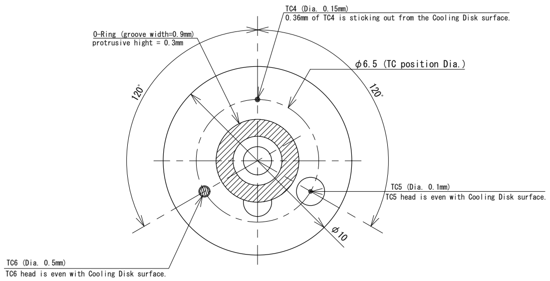
TC layout on Cooling Disk View from the heating disk side
