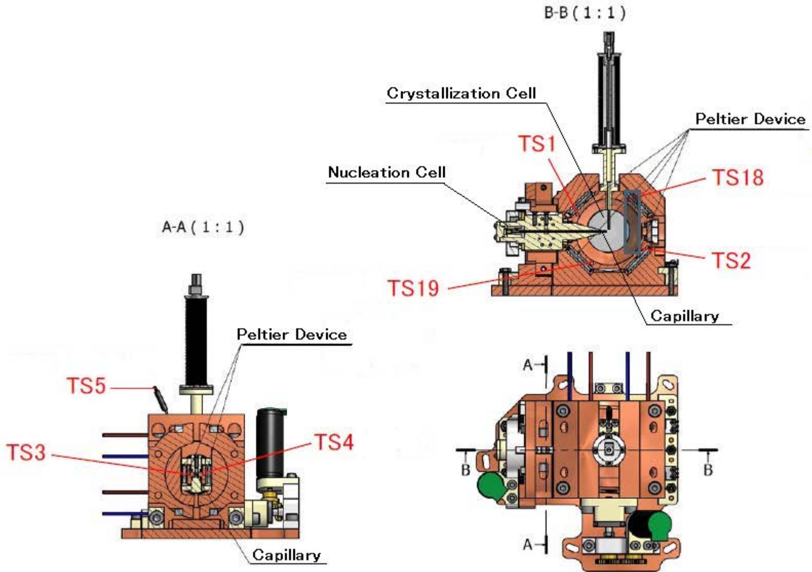
General Drawing of Ice 2 ( Crystallization Cell and Nucleation Cell )
