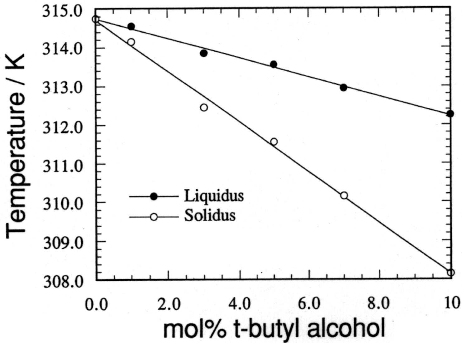
Phase Diagram
