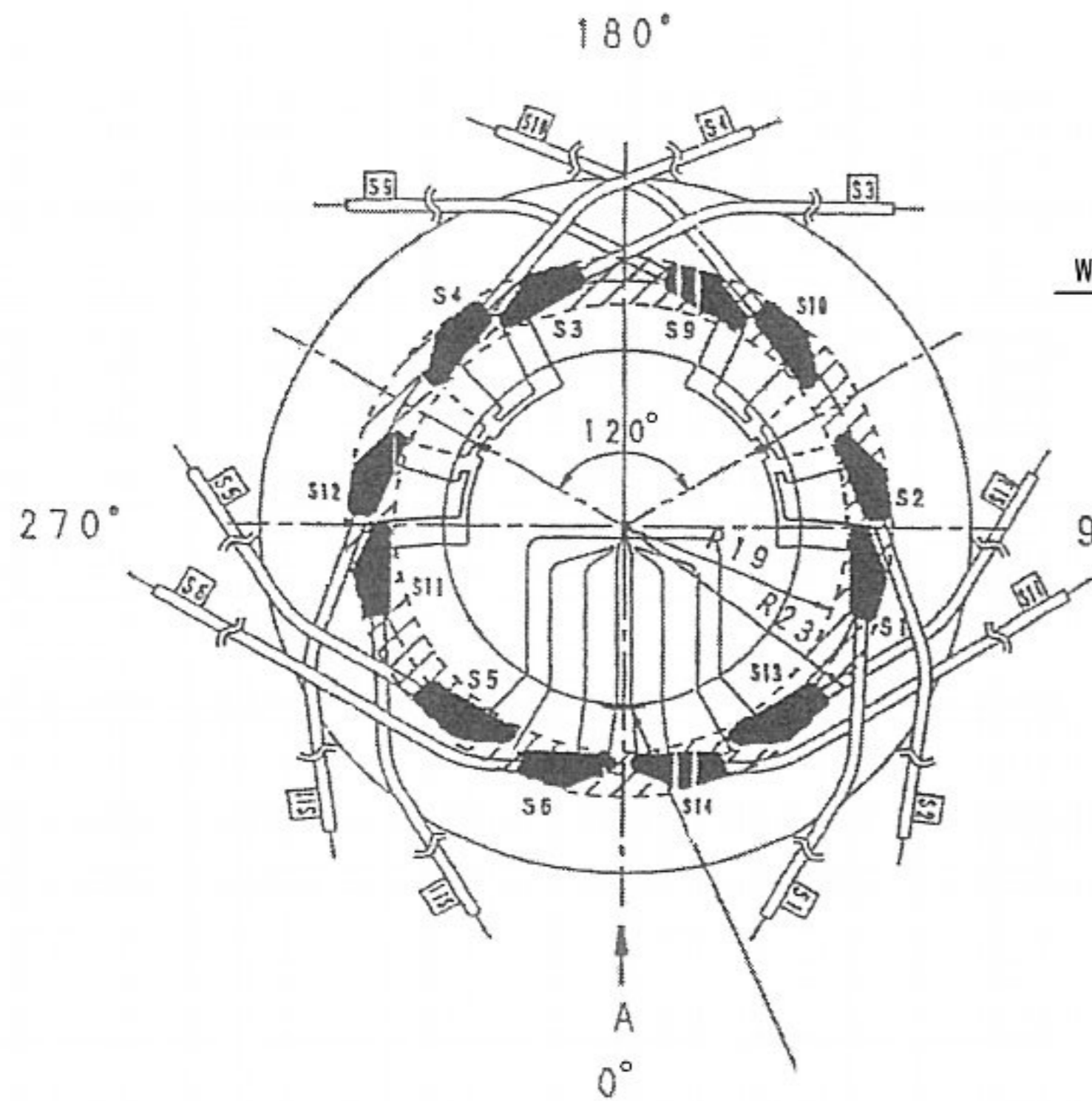
ITO sensor side
